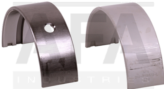
Main Bearing, Plain - STD 2110587 | Caterpillar | C11/C13/3196
